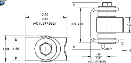
Slotted Yoke Allows For a 1/2" of Adjustment On Each Hinge.
